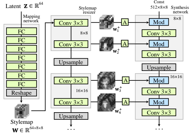
Figure 3: StyleMapGAN Generator. The stylemap w is resized to w^+ through convolutional layers to match the spatial resolution of each feature in the synthesis network. Here “A” stands for a learned affine transform, which produces spatial modulation parameters ( \gamma and \beta in Equation 1). “Mod” indicates modulation consisting of element-wise multiplication and addition. Note that the synthesis network starts from a learned constant input, and the output image’s style is adjusted by resized stylemaps.
