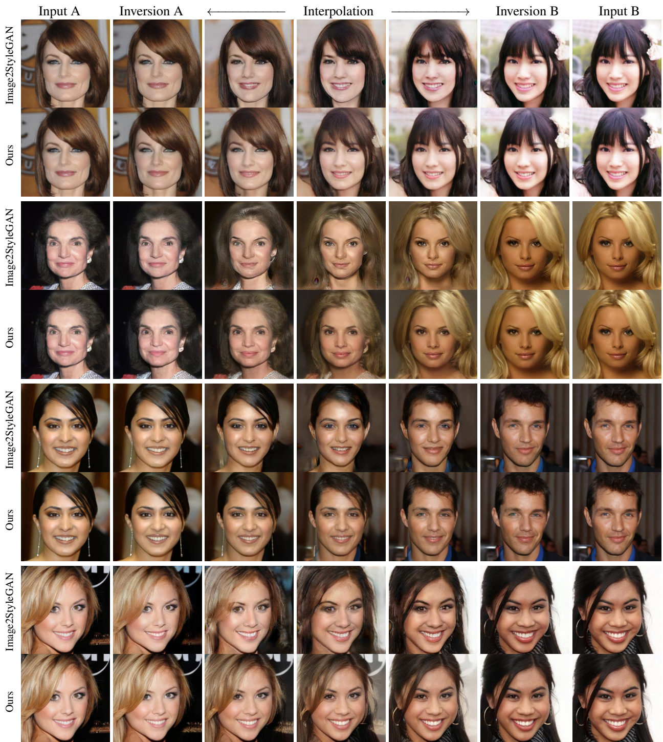
Figure 14: Comparison with Image2StyleGAN for interpolation quality. Image2StyleGAN shows rugged and discontinuous interpolations, even though the reconstruction quality is visually good. Our method produces clearer and smoother interpolations, which reveal our superiority in both pixel-level and semantic-level ( i.e. , the semantics the original latent space) reconstruction. Note that the reconstruction speed of our method is 2000\times faster than Image2StyleGAN.
